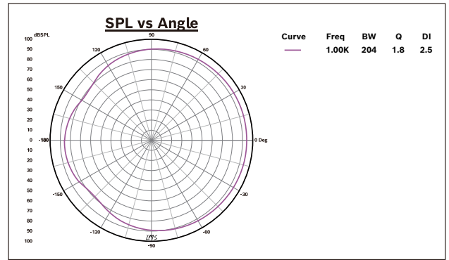
Fig. 3: Polar pattern diagram: 1K vertical directivity
