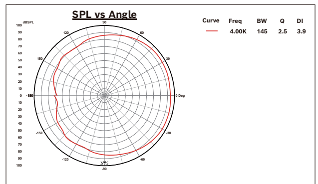
Fig. 5: Polar pattern diagram: 4K vertical directivity
