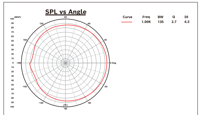
Fig. 4: Polar pattern diagram: 1K horizontal directivity
