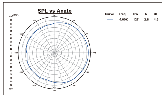
Fig. 6: Polar pattern diagram: 4K horizontal directivity
